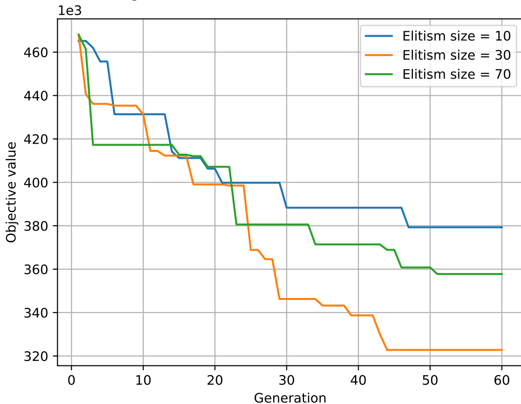
GA convergence for different elitism sizes (median over runs)
